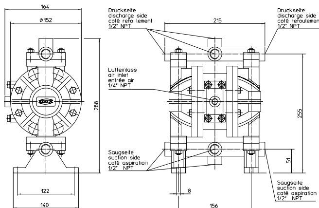
Dimensions [mm]
