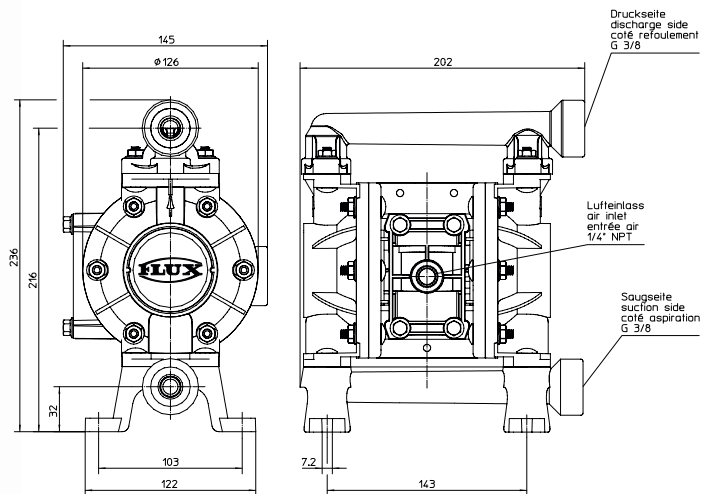
Dimensions [mm]
