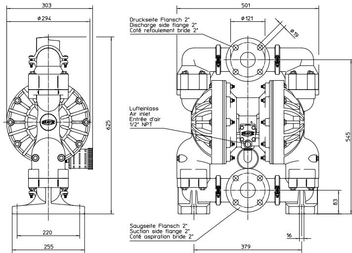
Dimensions [mm]
