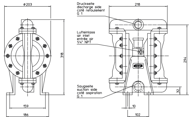
Dimensions [mm]
